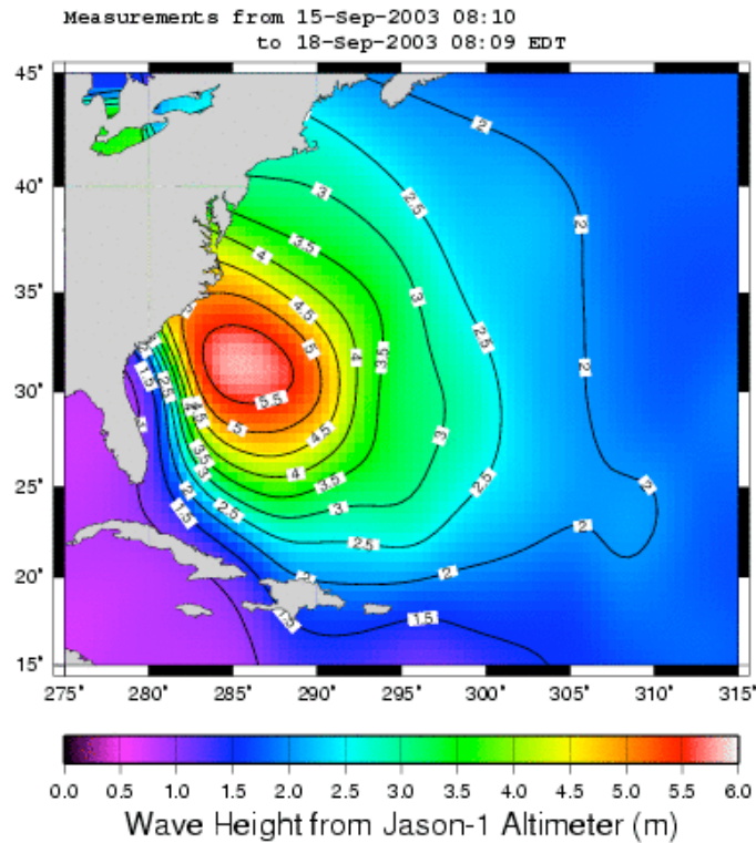
Jason significant wave height data during Hurricane Isabel, September 2003.
