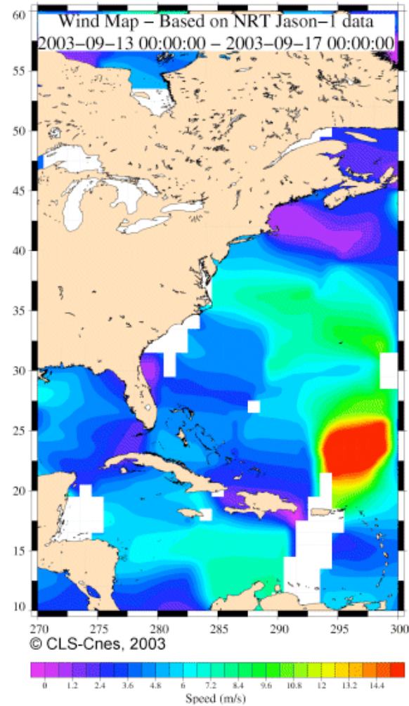
Wind data from Jason NRT data during Hurricane Isabel, September 2003.
